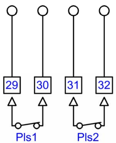
Figure 2.3 Pulse Output Connection
