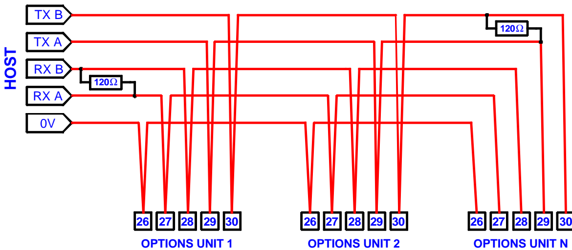
Figure 5.5 RS422 Multi-Drop Connection
