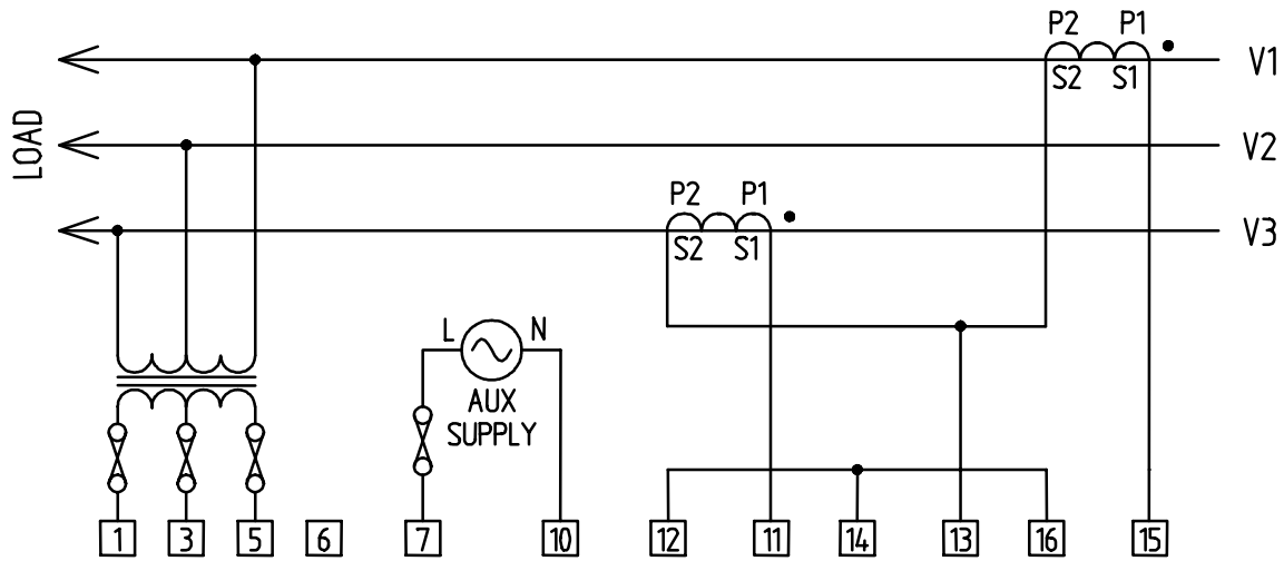
Figure 3.6 3 Phase 3 Wire Using Potential Transformers
