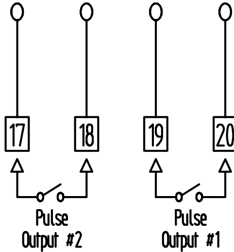
Figure 2.2 Pulse Output Connection
