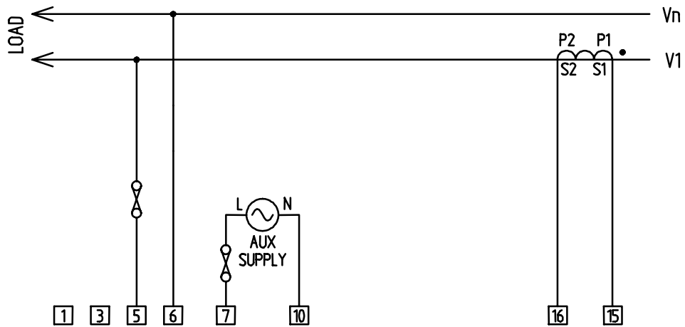
Figure 3.5 Single Phase
