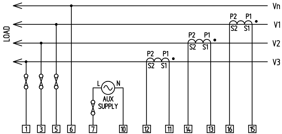
Figure 3.4 3-Phase 4-Wire
