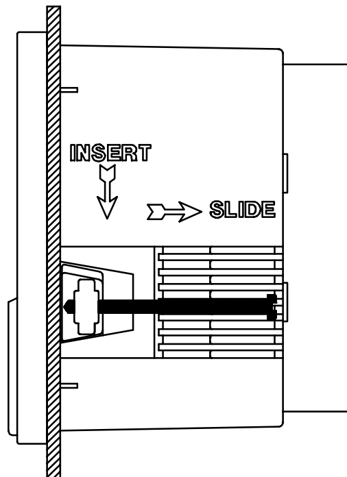
Figure 3.1 Fitting The Meter in a Panel
