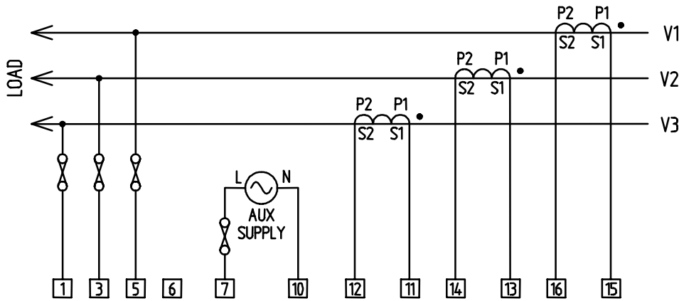
Figure 3.3 3-Phase 3-Wire 3CTs
